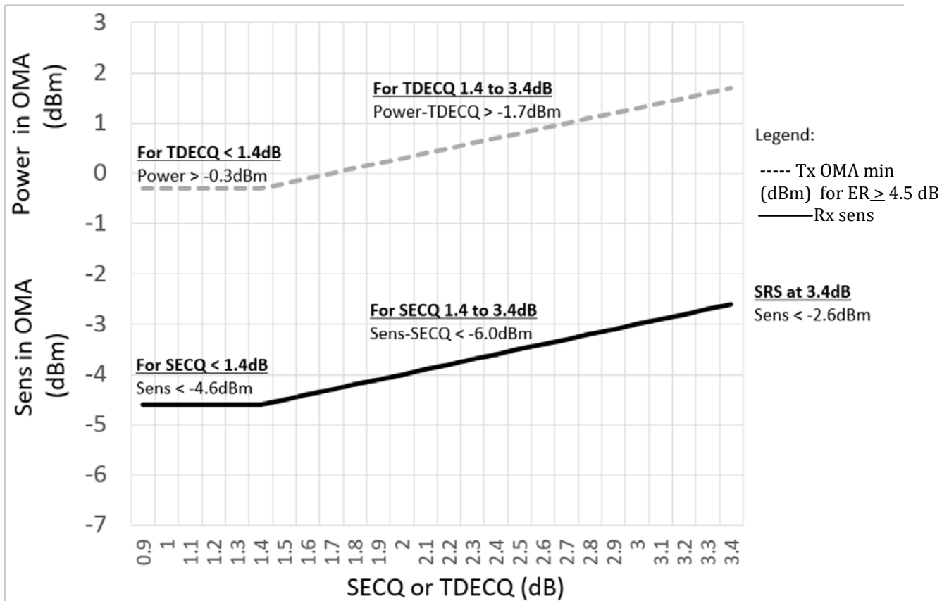
Figure 2-1 Illustration of receiver sensitivity mask for 400G-FR4
