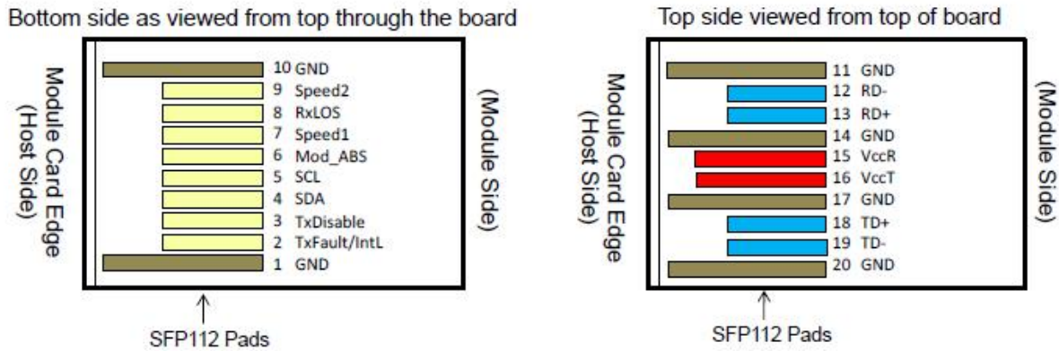
Figure 3. Pin View
